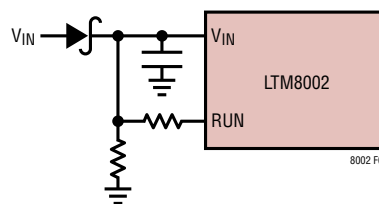
Figure 4. The Input Diode Prevents a Shorted Input from Discharging a Backup Battery Tied to the Output. It Also Protects the Circuit from a Reversed Input. The LTM8002 Runs Only When the Input Is Present
